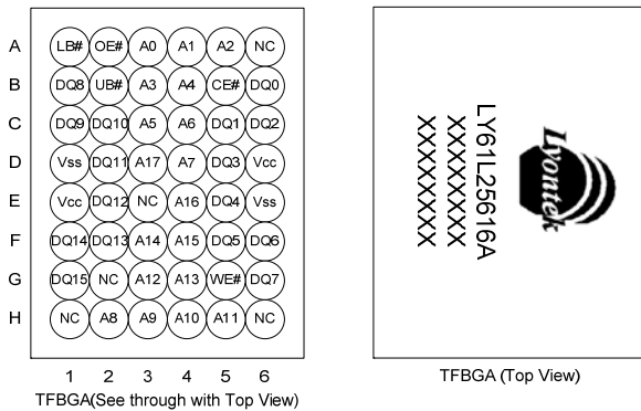
TFPGA(See through with Top View)
