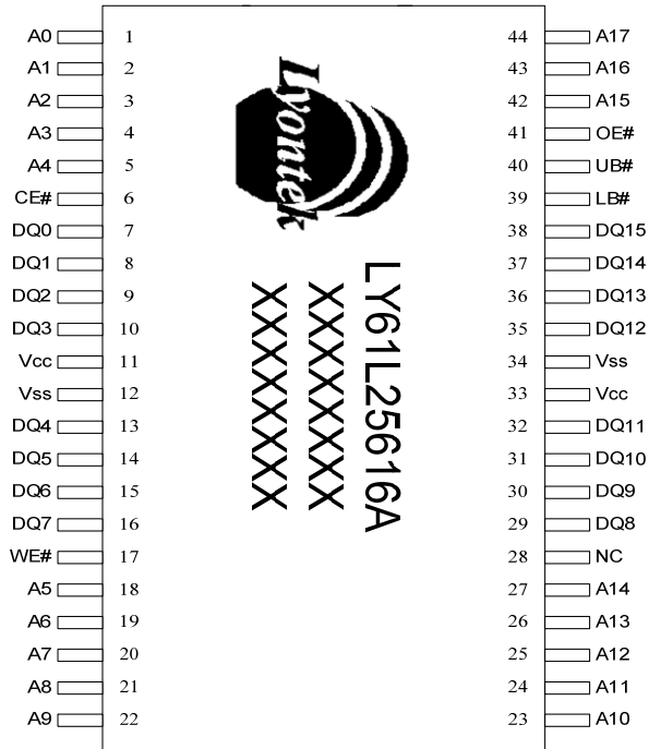
TSOP II
