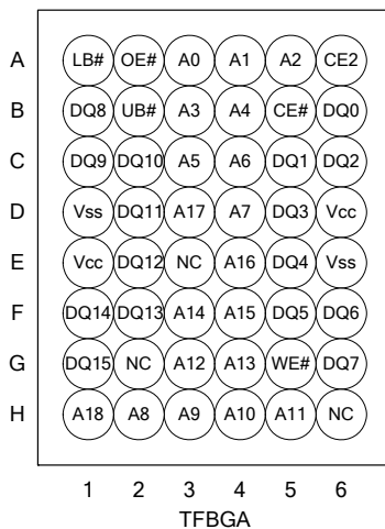
TFBGA
